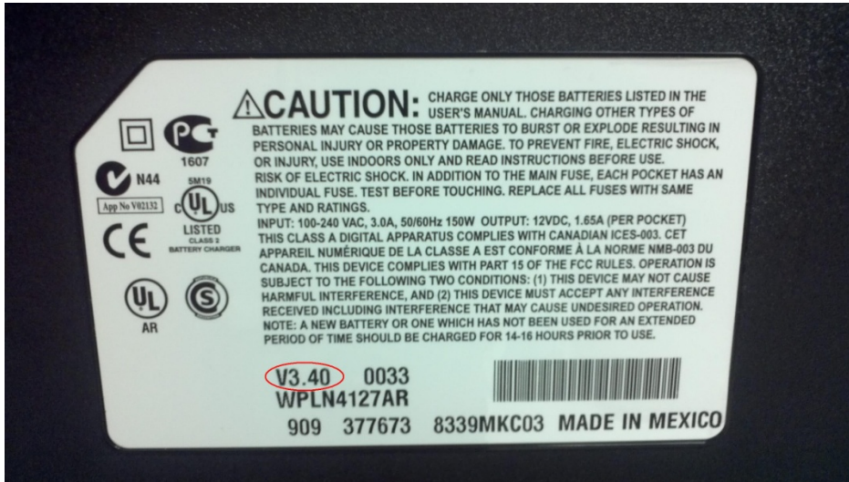
Figure 1: XTS Multi-Unit charger
